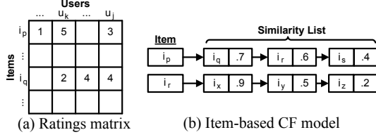
Fig. 2. Item-based CF model generation.
