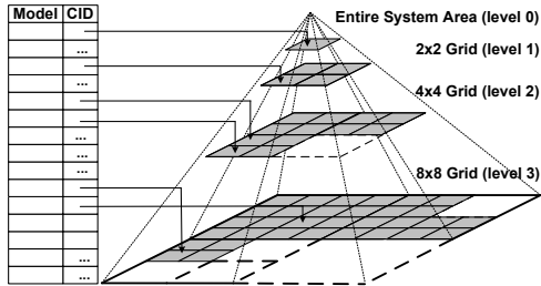
Fig. 4. Partial pyramid data structure.
