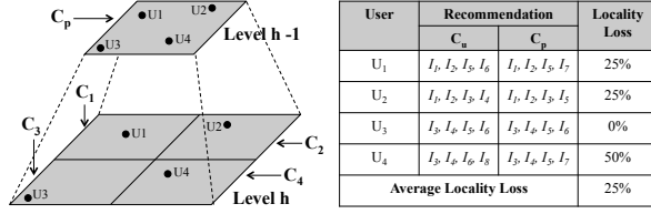
Fig. 5. Merge and split example.
