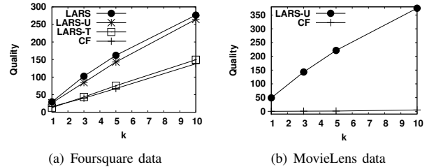
Fig. 7. Quality experiments for varying answer sizes
