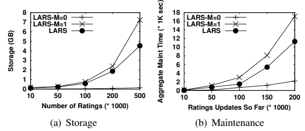
Fig. 9. Scalability of the adaptive pyramid
